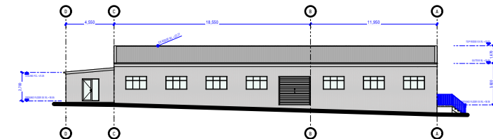
4 EAST ELEVATION
