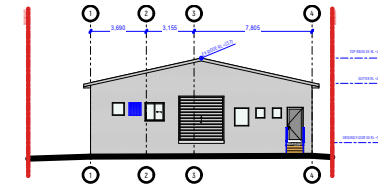
1 NORTH ELEVATION
