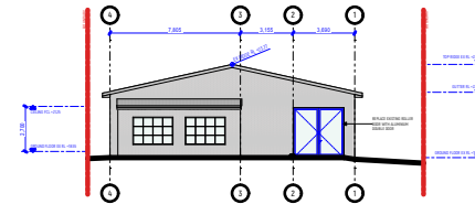
3 SOUTH ELEVATION
